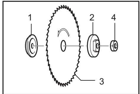
► 1. Inner flange 2. Outer flange 3. Saw blade 4. Hex nut
