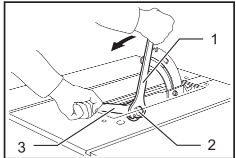
► 1. Wrench 2. Hex nut 3. Offset wrench
