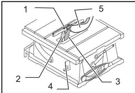
► 1. Table saw blade guard assembly 2. Antikickback pawls 3. Riving knife/spreader 4. Riving knife/spreader release lever location 5. Table saw blade side guards
