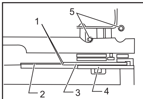
► 1. These two clearances should be equal 2. Blade 3. Riving knife/spreader 4. Pressure plate 5. Hex bolts
