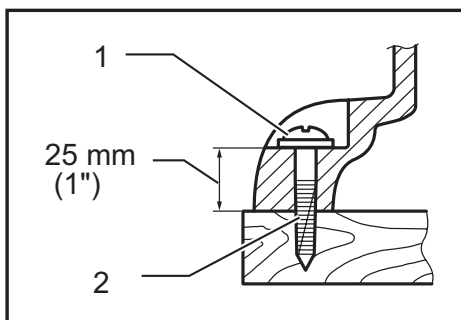
► 1. 6 mm (1/4") Std. washer 2. No.10 wood screw 40 mm (1-1/2") min. length
