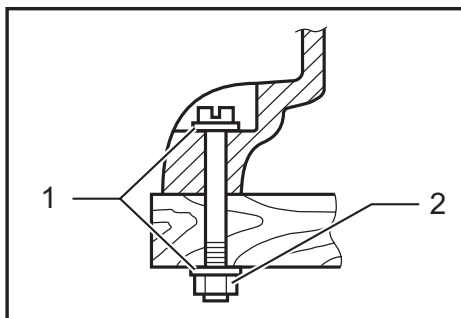
► 1. 6 mm (1/4") Std. washer 2. 6 mm (1/4") Mounting bolt & Nut tighten securely
