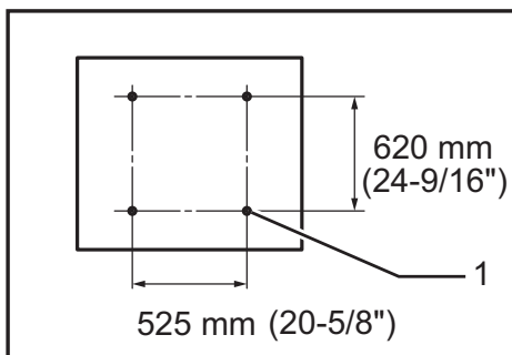
► 1. Hole diameter 8 mm (5/16")
